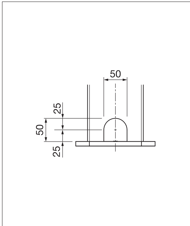
W3 = Support with Drainage hole
